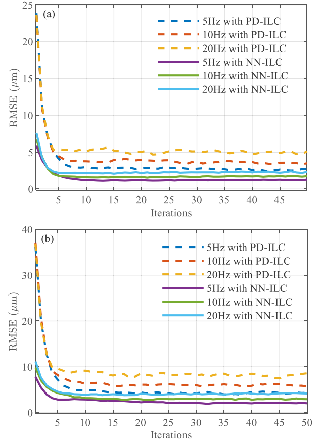
Fig. 10. Iterative process of the RMSE with PD-ILC and NN-ILC under three frequencies. (a) Sinusoidal cases. (b) Triangular cases.
