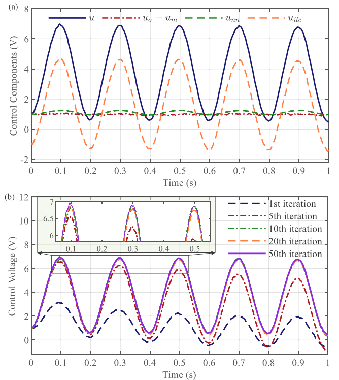
Fig. 6. Components and evolution analysis of the control voltage. (a) Control components of the NN-ILC controller in the last iteration. (b) The evolution process of the control voltage for NN-ILC during the iterations.
