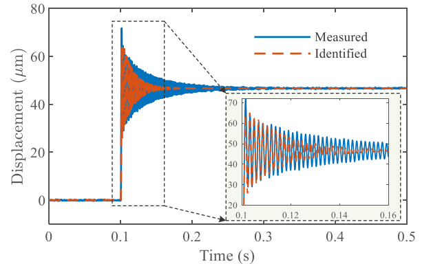
Fig. 4. Step responses of the measured data and simulated data of the identified model.
